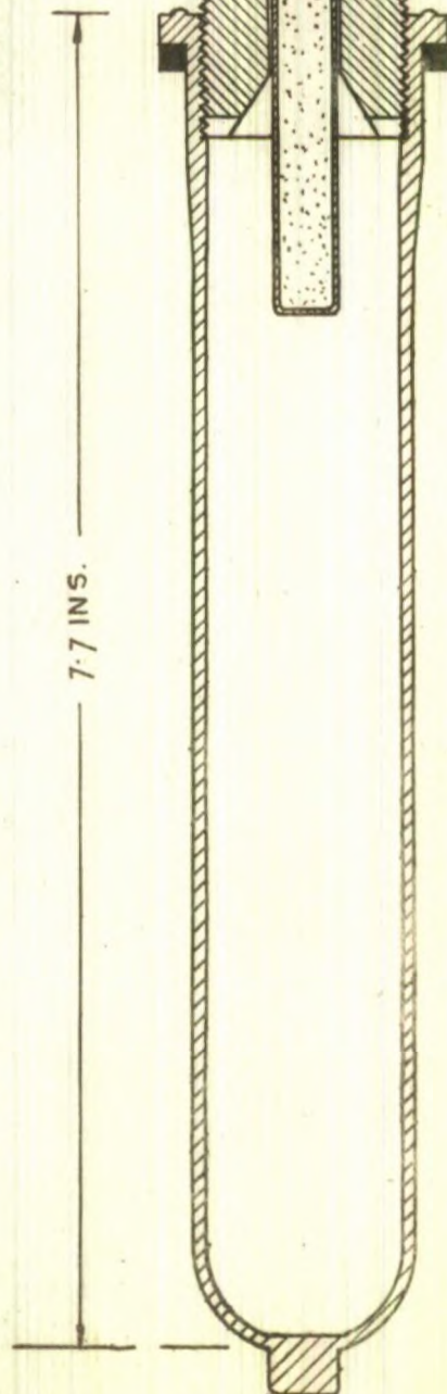
LONG GAINE.
