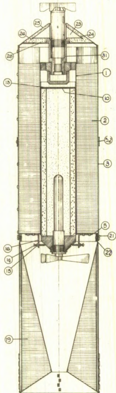
SECTION C.C.
