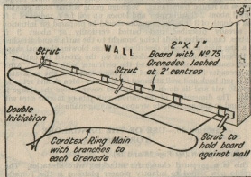
Fig 17. Demolishing a 9-inch brick wall
