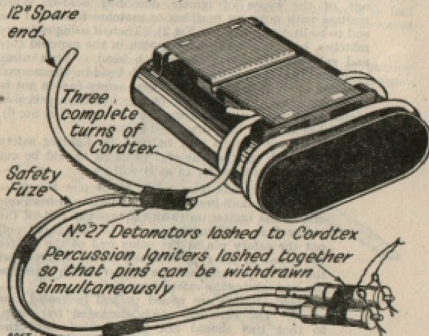
Fig 6. No. 75 grenade prepared as a demolition charge
