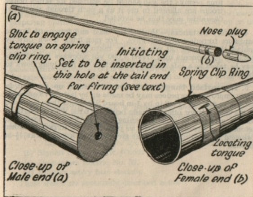
Fig 19. 1½ in. bangalore torpedo, Mk. 1
