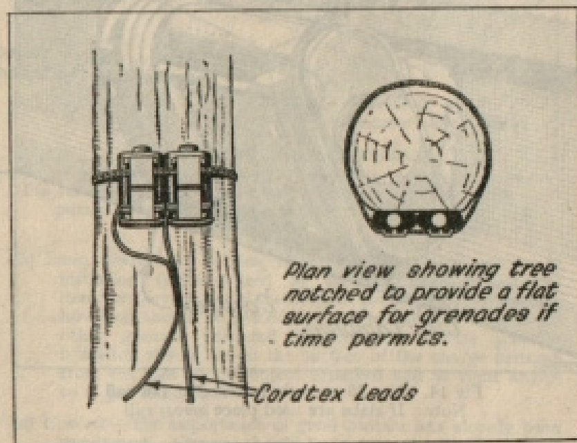
Fig 15. Tree felling using 75 grenades
