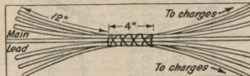
Fig 10. Cordtex junction box
