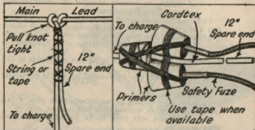
Fig 7. Cordtex clove hitch joint
