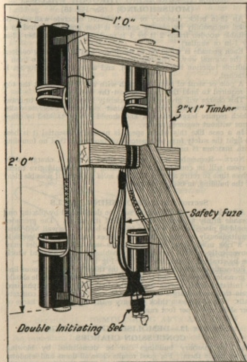
Fig 16. Pole charge for "mouseholing"
