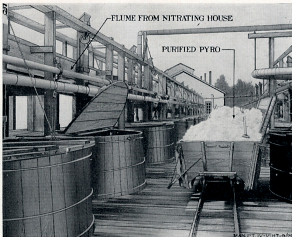
FIGURE 7.—Boiling tubs.
