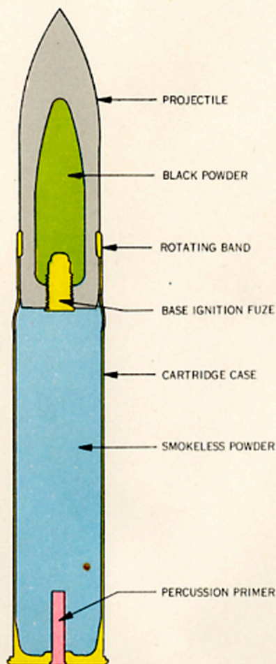
FIG. 1—COMMON (COMPLETE ROUND)
