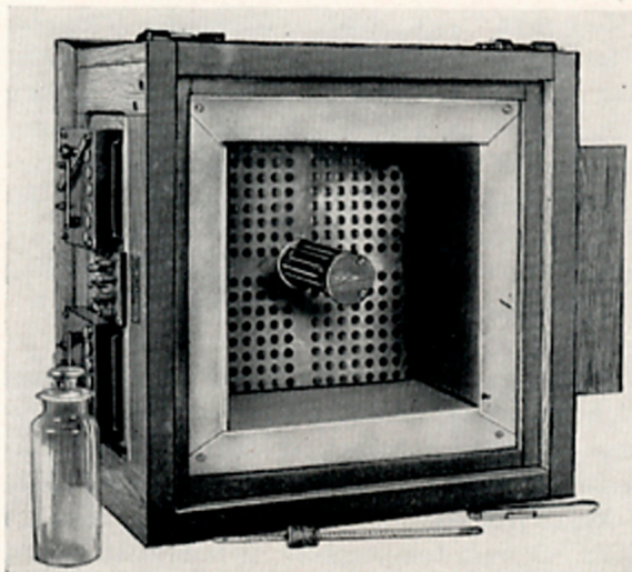
FIGURE 23.—Mark 2 oven interior.
