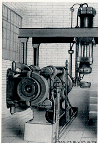
FIGURE 16.—Graining press.
