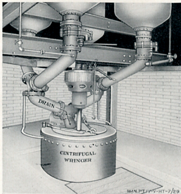
FIGURE 5.—Centrifugal wringer.
