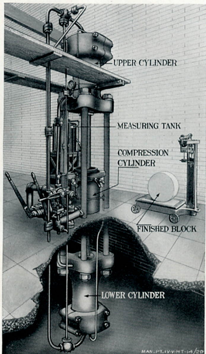
FIGURE 12.—Dehydrating press.
