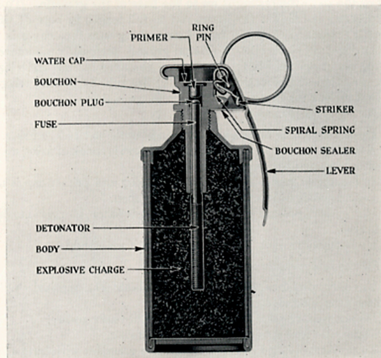
FIGURE 36.—Cross section of a hand grenade.
