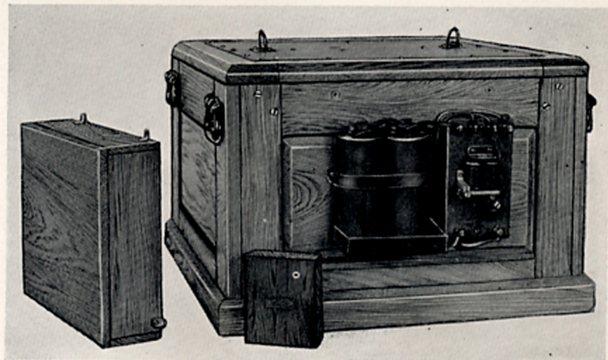
FIGURE 21.—Mark 2 oven showing relay.
