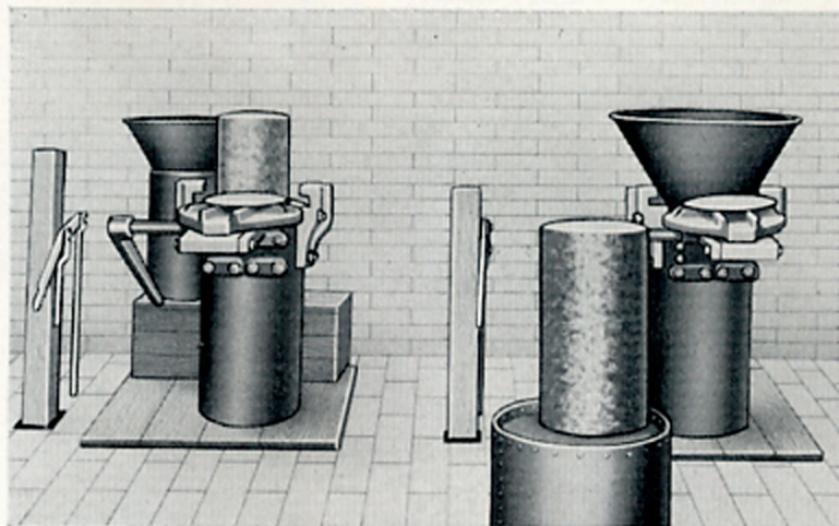
FIGURE 14.—Blocking press.
