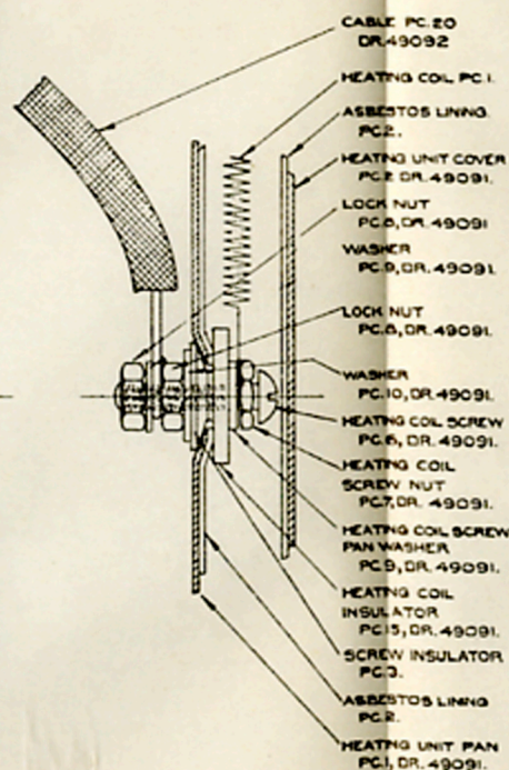
TYPICAL SECTION THROUGH HEAT UNIT.
