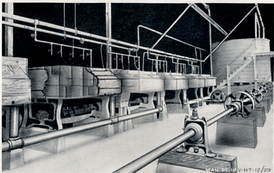
FIGURE 10.—Pyro screens.
