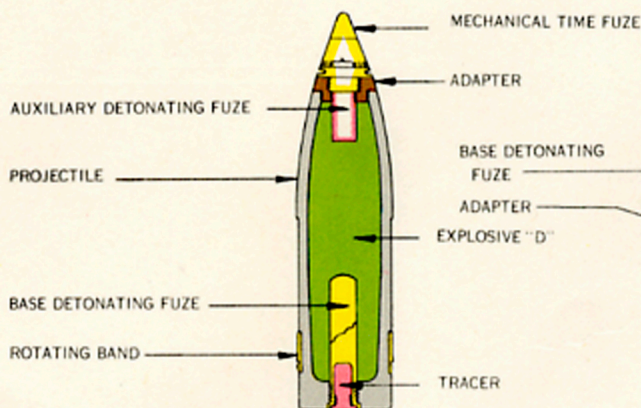
FIG. 2.—ANTI-AIRCRAFT COMMON
