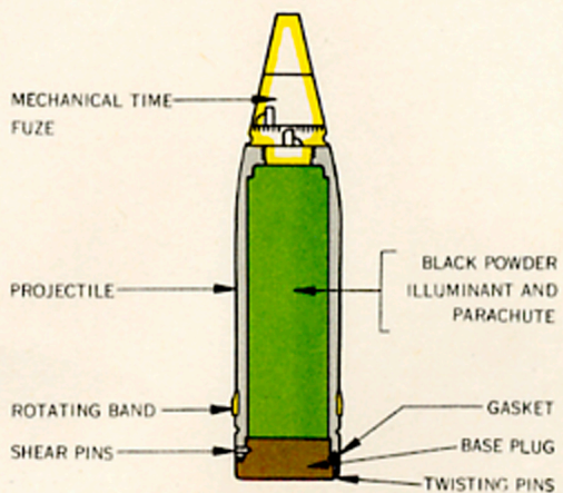
FIG. 3.—ILLUMINATING
