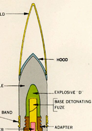
FIG. 4.—SPECIAL COMMON
