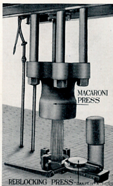
FIGURE 15.—Macaroni press.
