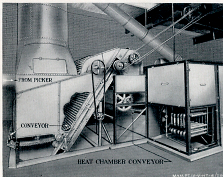
FIGURE 3.—Cotton dryer.
