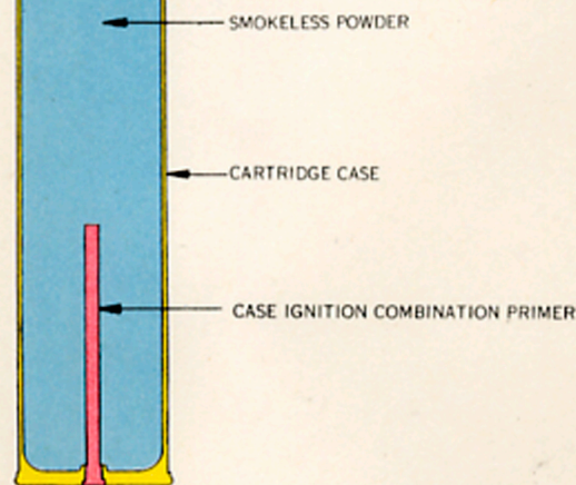
FIG. 1.—COMMON (COMPLETE ROUND)
