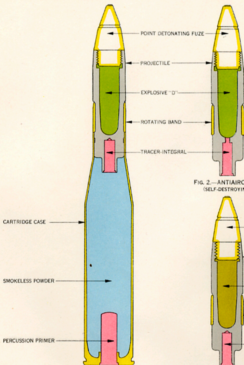
FIG. 1.—ANTI-AIRCRAFT (COMPLETE ROUND)
