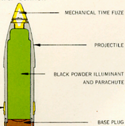
FIG. 4.—ILLUMINATING
