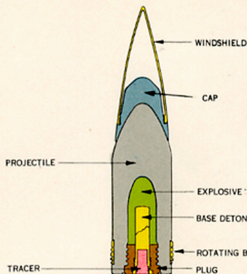
FIG. 2.—ARMOR PIERCING
