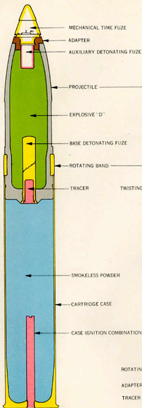
FIG. 1.—ANTI-AIRCRAFT (COMPLETE ROUND)
