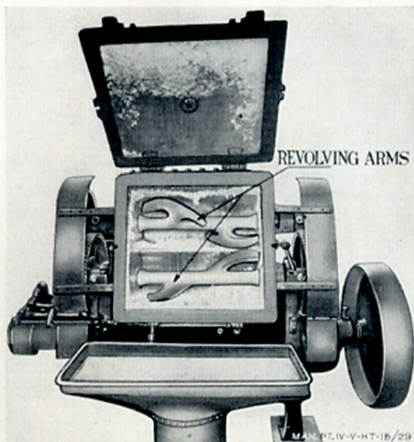
FIGURE 13.—Mixing machine.
