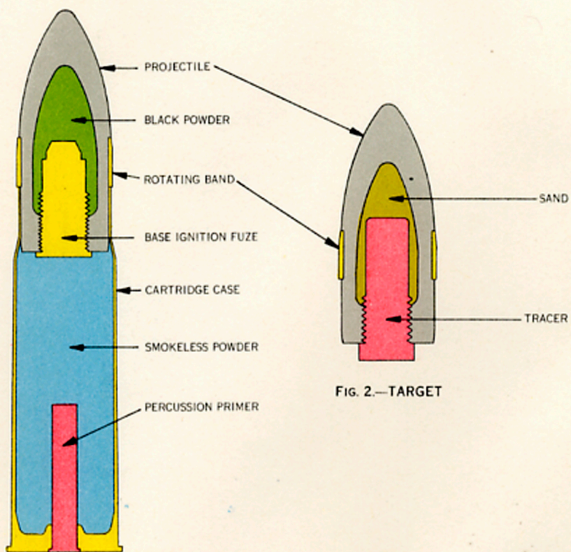
FIG. 1—COMMON (COMPLETE ROUND)
