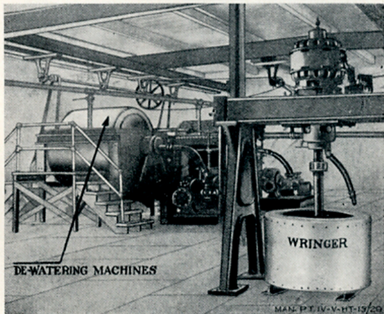
FIGURE 11.—Dewatering machine.
