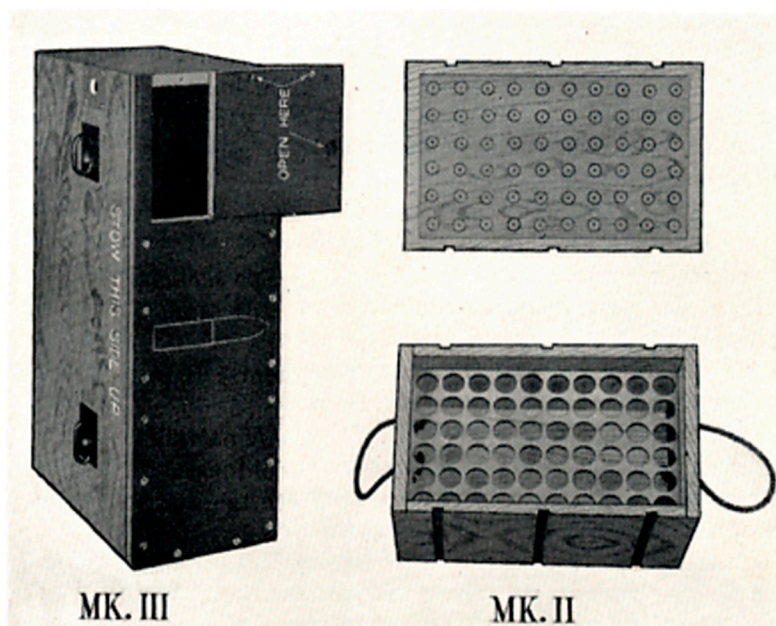
FIGURE 25.—1-pounder ammunition boxes, Marks 2 and 3.
