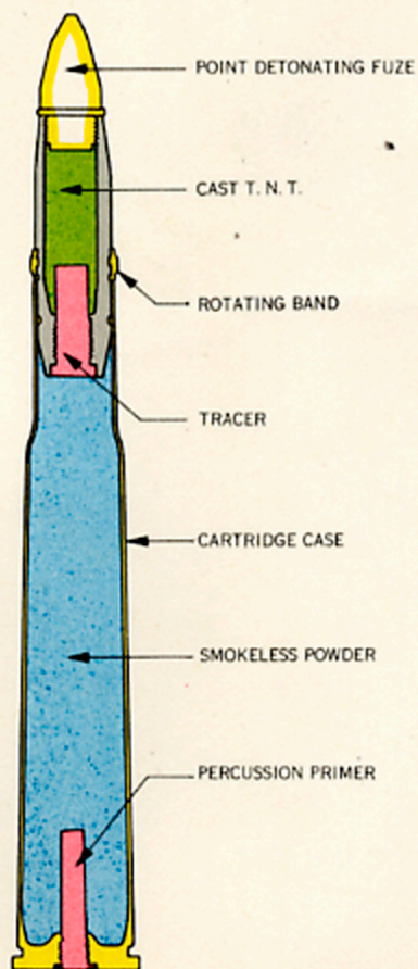
FIG. 1.—ANTI-AIRCRAFT (COMPLETE ROUND)
