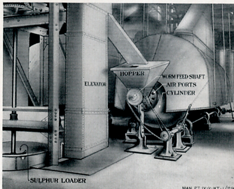
FIGURE 1.—Sulphur burner.
