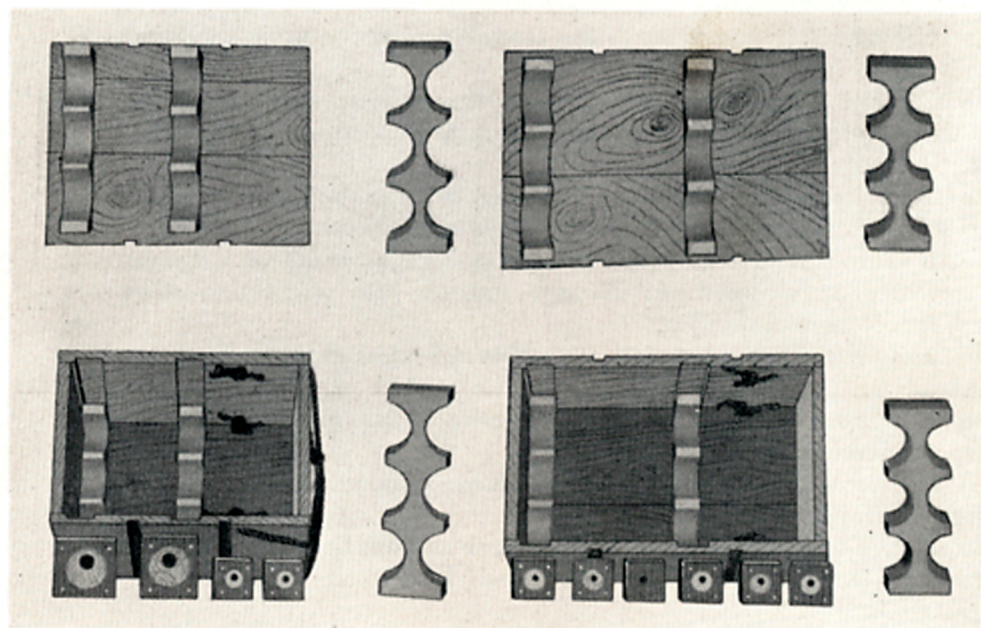
FIGURE 26.—3 1/2 inch 23 caliber ammunition boxes, Mark 4 and 4 Mod. I.
