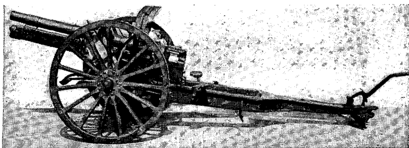
Figure 9.—Model 38 (1905) 75-mm gun improved, left side.
