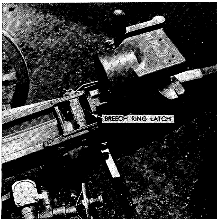
Figure 93. Fourth step: (2) removal of the breech.
