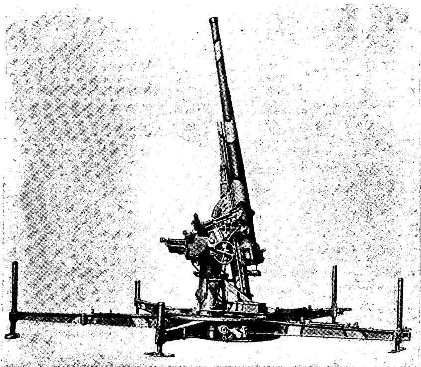
Figure 17. Model 88 (1928) 75-mm AA gun, emplaced.
