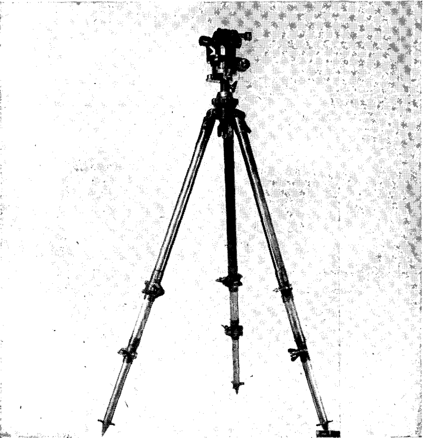
Figure 84. Aiming circle.
