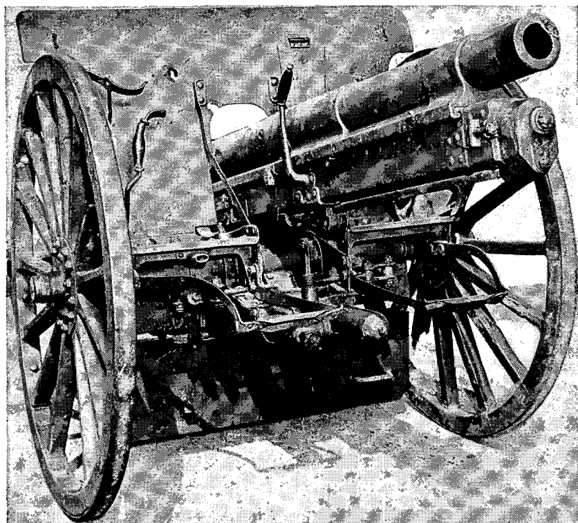
Figure 11.—Model 38 (1905) 75-mm gun improved, showing equilibrators.
