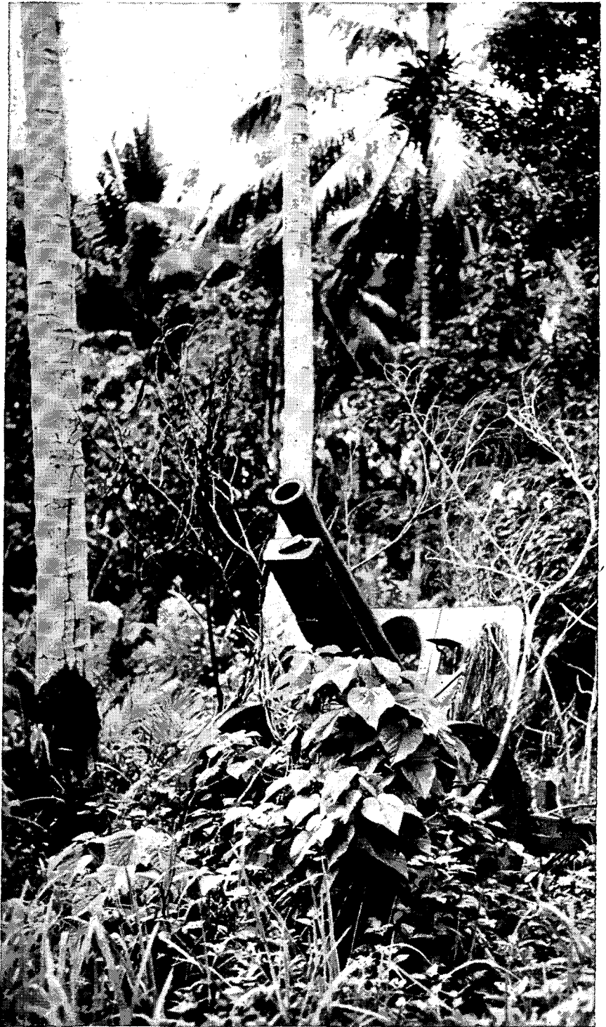
Figure 62. Model 96 (1936) 150-mm howitzer emplaced in the jungle. The tube is in full recoil.
