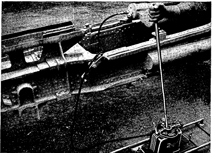
Figure 115. Rear end of cradle showing the M3 liquid pump attached for adding the recoil mechanism liquid.
