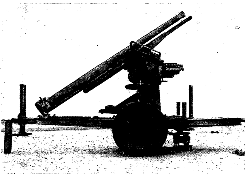
Figure 18. Model 88 (1928) 75-mm AA gun in traveling position.
