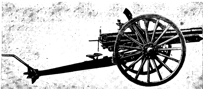
Figure 26. Model 41 (1908) 75-mm cavalry gun.
